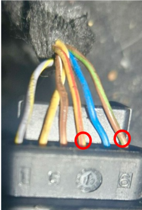
Figure 2a - Sensor at the accelerator pedal
