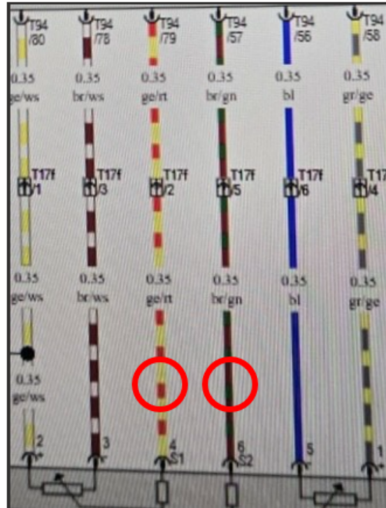
Figure 2b - Wiring diagram of sensor (wires are not in same order as actual sensor)
