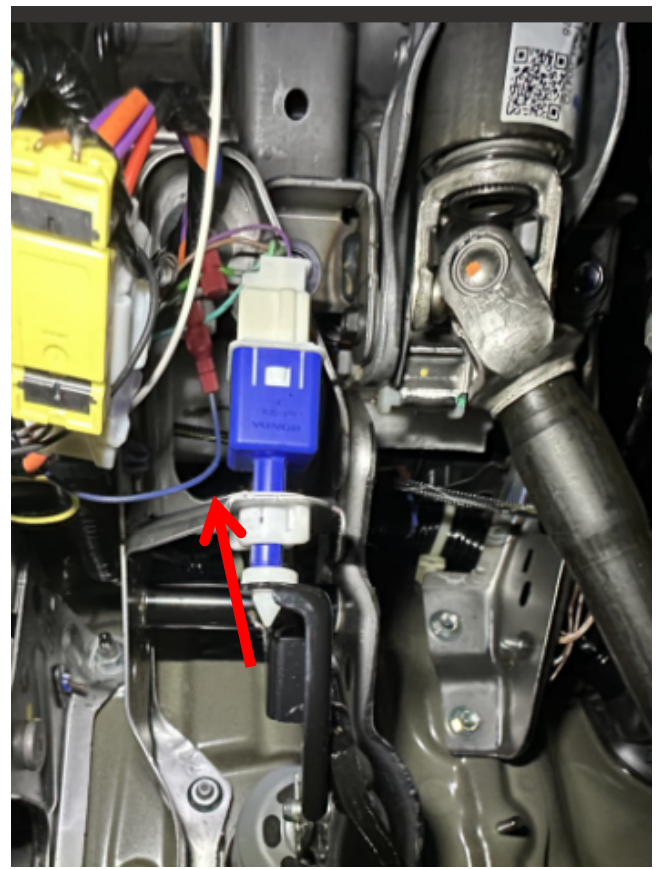
Figure 4 (Brake Sensor)
