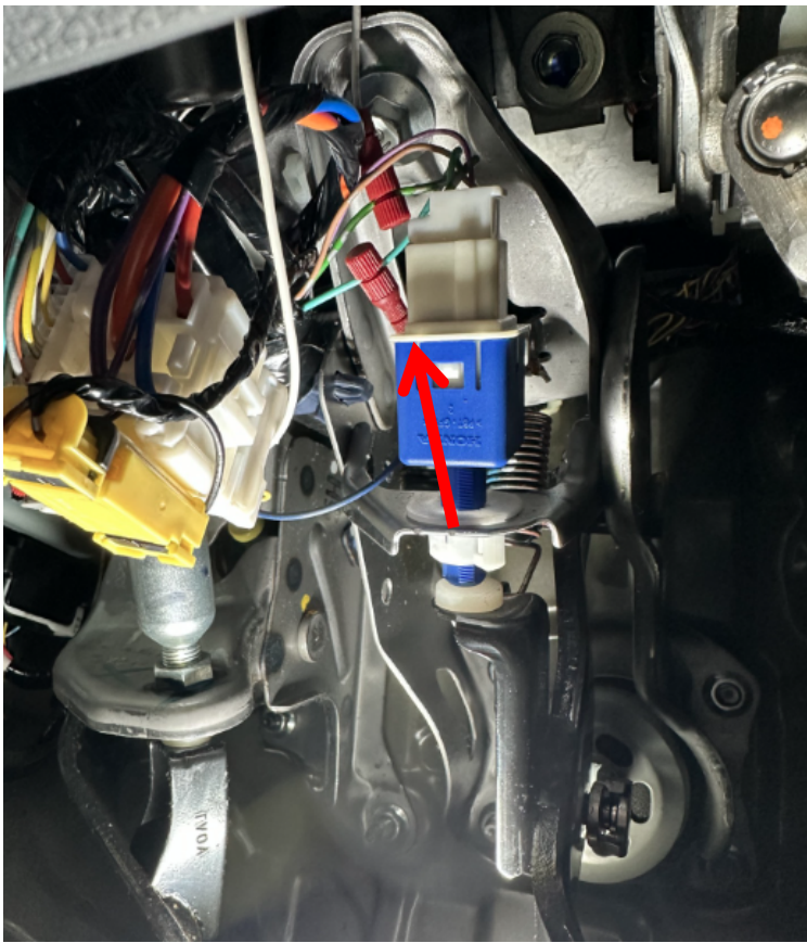
Figure 4 (Brake Sensor)
