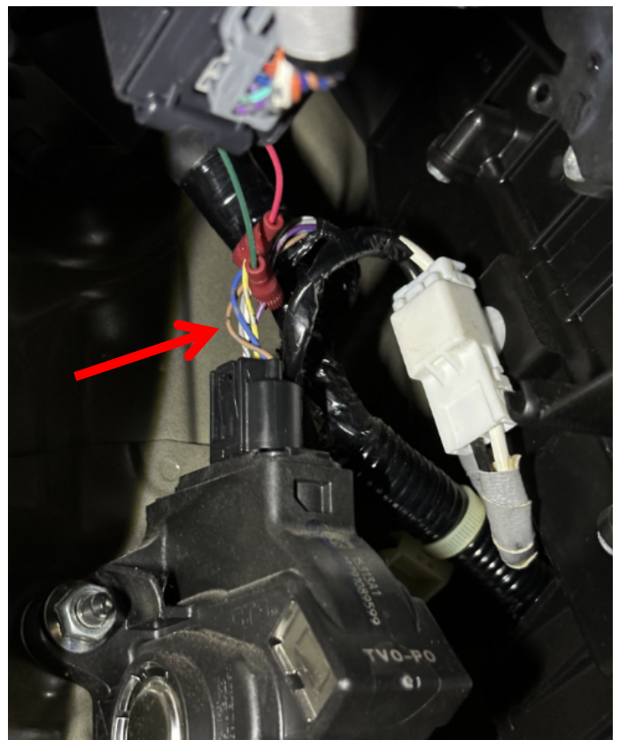
Figure 5 (Accelerator Pedal Position Sensor)
